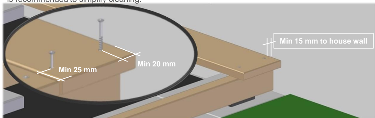
Figure 3: Distance from building & screw positions
