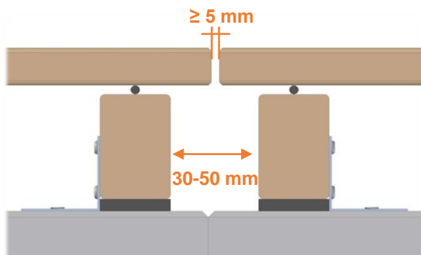
Figure 5: Decking board with EPDM pads over 2 beams. This method increases longevity and simplifies cleaning.
