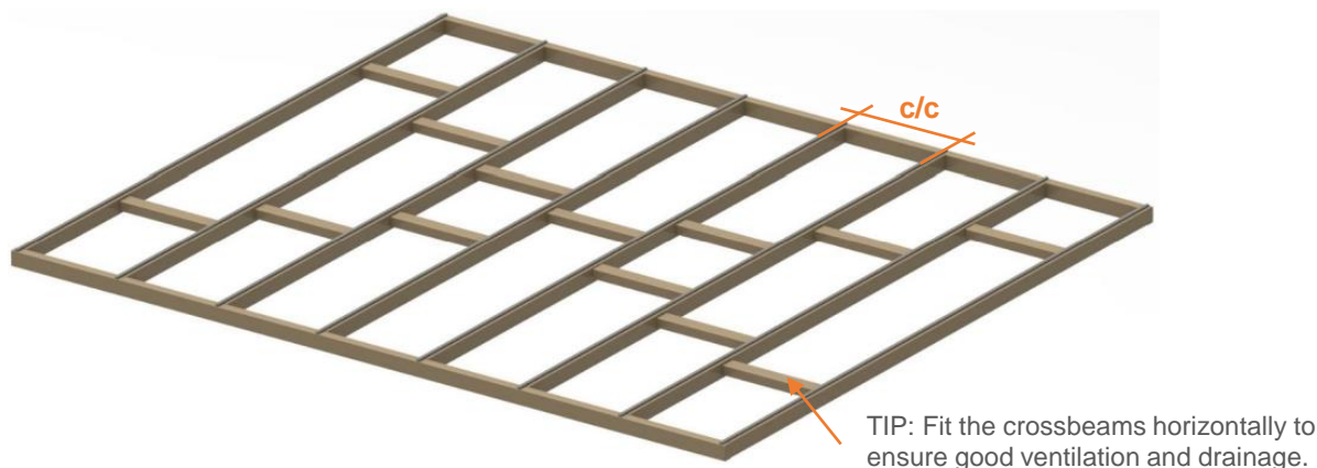
Figure 6: Example of stiffening of joist layer.
