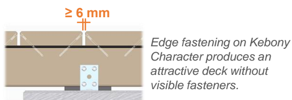
Figure 1: Edge fastening of Kebony Character Decking
