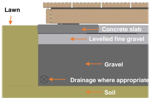
Figure 9: Substrate Design
