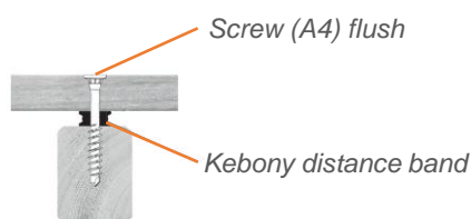
Figure 2: Kebony Distance Band
